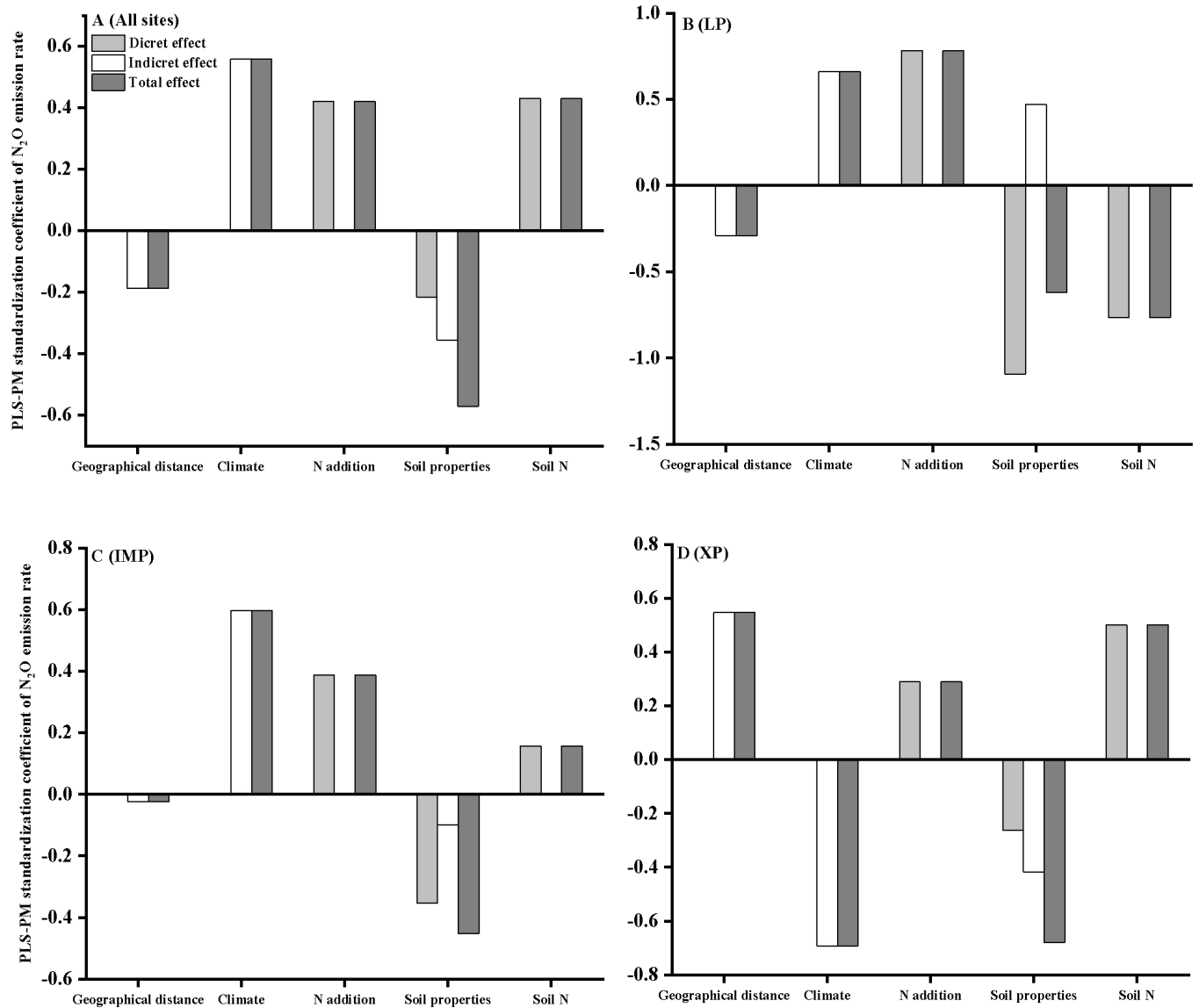
Supplementary Fig. S1 Standardized coefficient direct, indirect and total effects derived from the PLS-PMs of soil N 2 O emission rates in all sampling sites at regional scale (A), and at sb-regional scale LP (B), IMP (C) and XP (D). LP- Loess Plateau, IMP- Inner Mongolia Plateau, XP- Xizang Plateau.
