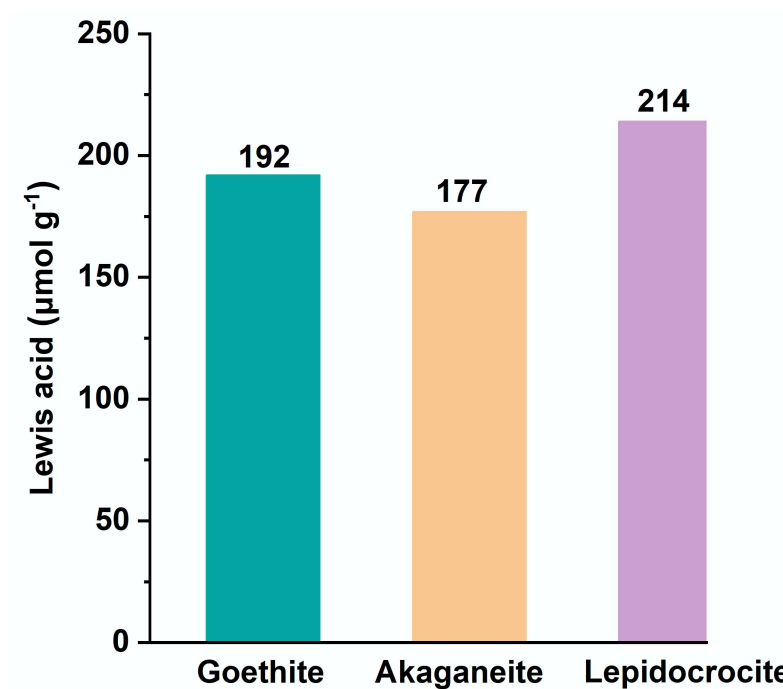
Supplementary Fig. S18 The Lewis acid content of goethite, akaganeite, and lepidocrocite as determined using Py-IR.
