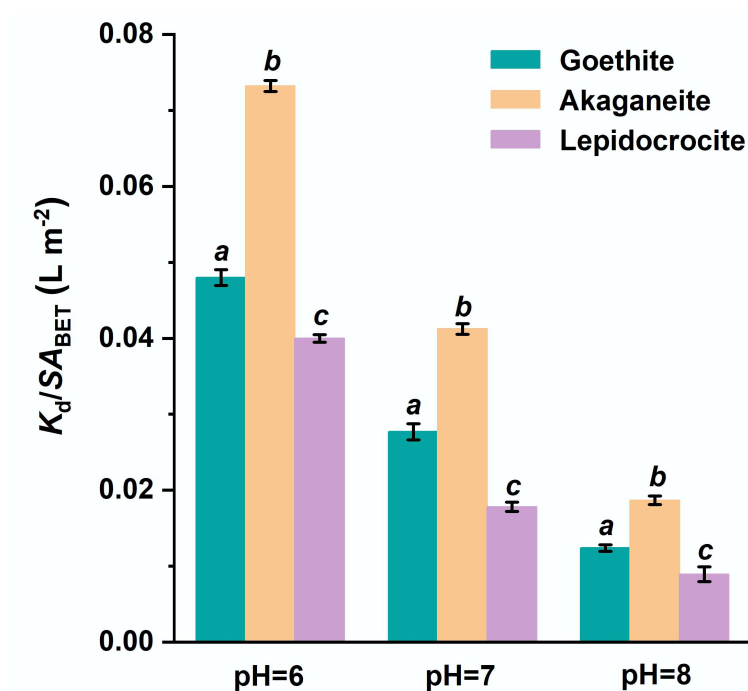
Supplementary Fig. S17 The surface area-normalized adsorption coefficients ( K_d ) of orthophosphate ion by the materials at different pH. Different letters denote significant differences ( p < 0.05 ).
