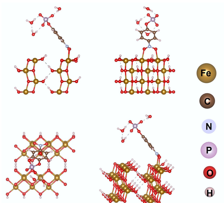
Supplementary Fig. S16 Structural models after the adsorption of pNPP on lepidocrocite via the -\text{NO}_2 group.
