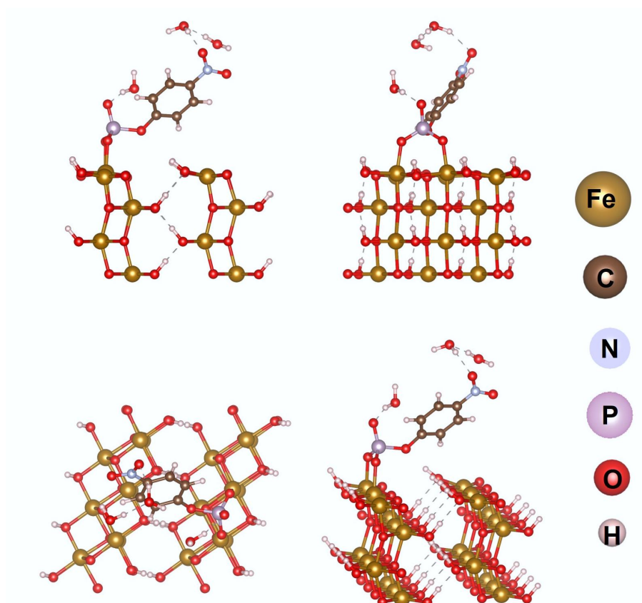
Supplementary Fig. S15 Structural models after the adsorption of pNPP on lepidocrocite via the -\text{PO}_4 group.
