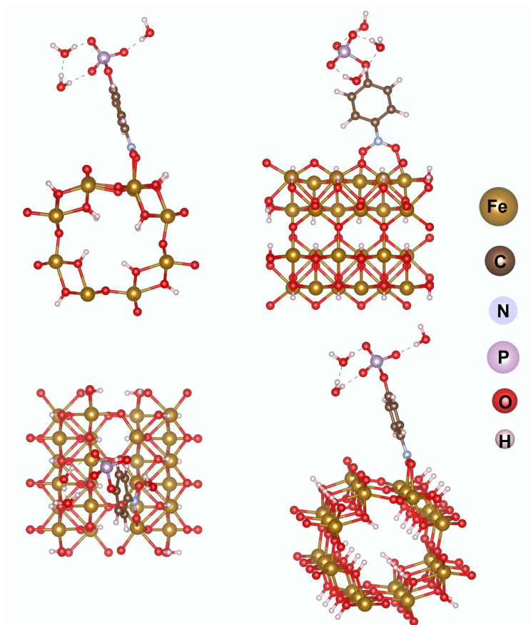
Supplementary Fig. S14 Structural models after the adsorption of pNPP on akaganeite via the -\text{NO}_2 group.
