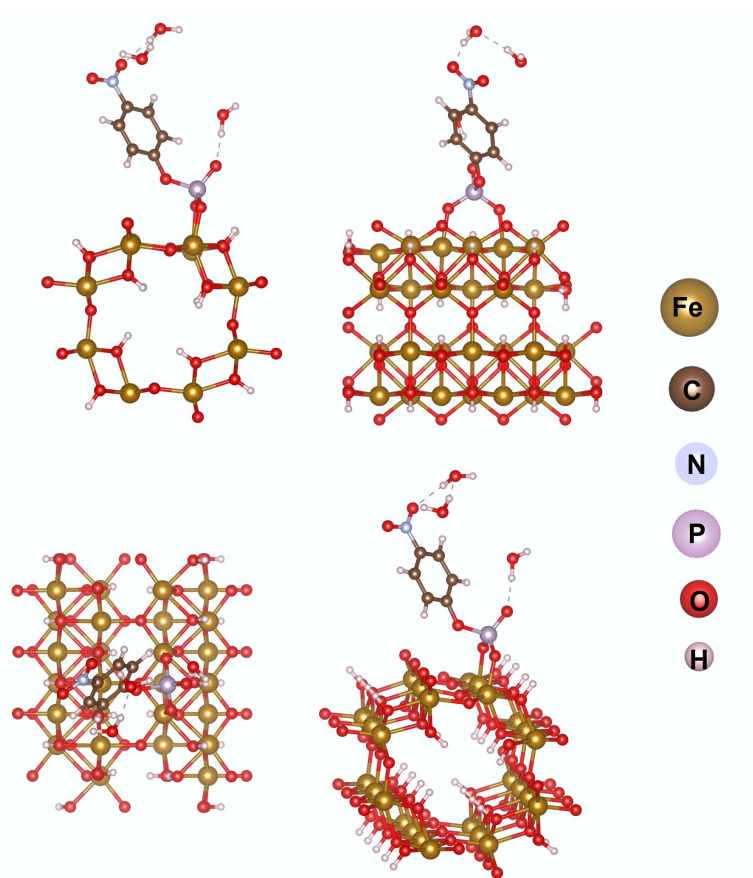
Supplementary Fig. S13 Structural models after the adsorption of pNPP on akaganeite via the -\text{PO}_4 group.
