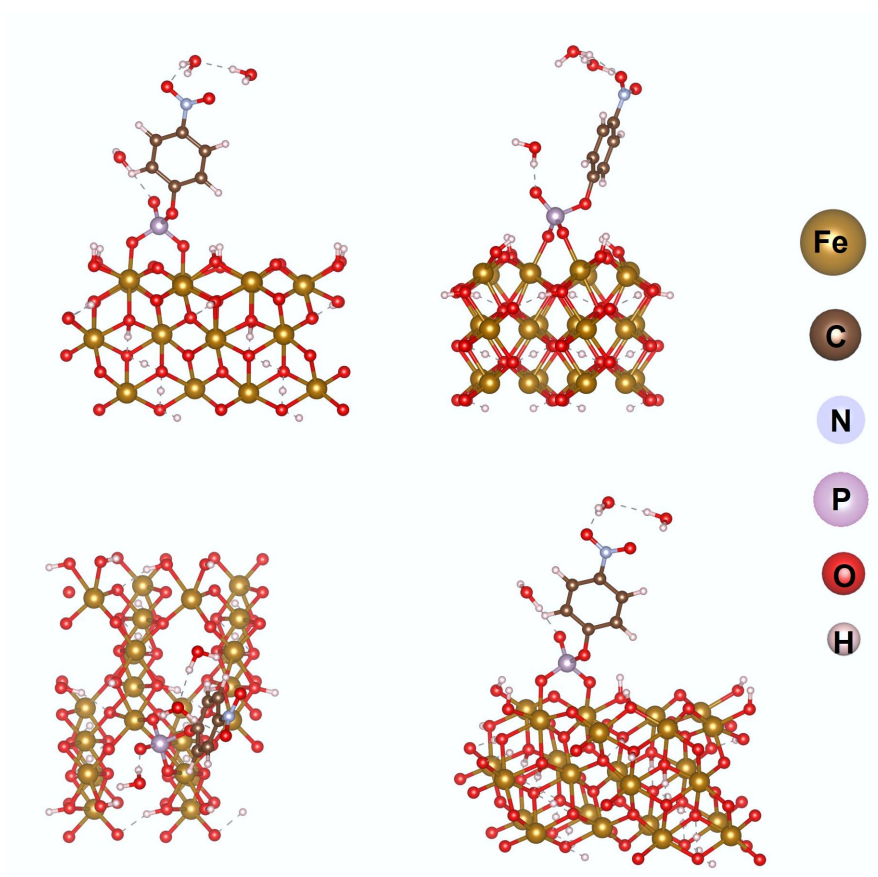
Supplementary Fig. S11 Structural models after the adsorption of pNPP on goethite via the -\text{PO}_4 group.
