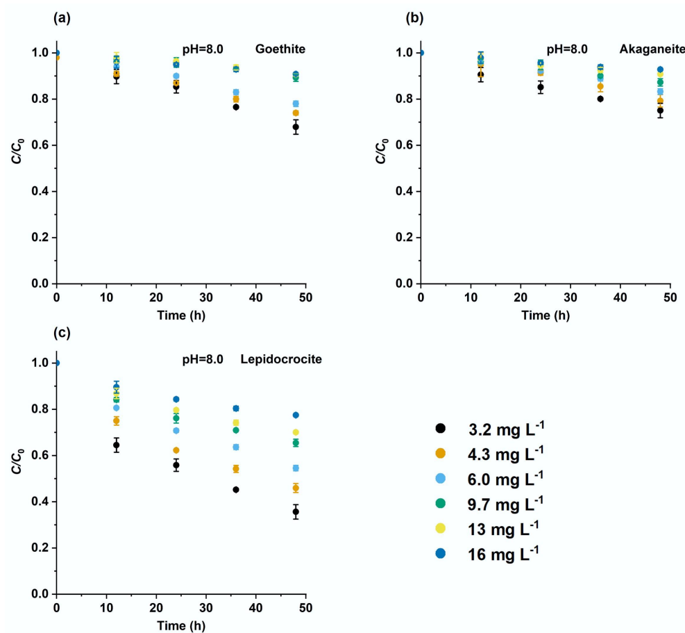
Supplementary Fig. S9 Catalytic hydrolysis kinetics of pNPP with different initial concentrations by different nanomaterials: (a) goethite, (b) akaganeite, and (c) lepidocrocite at pH 8.0.
