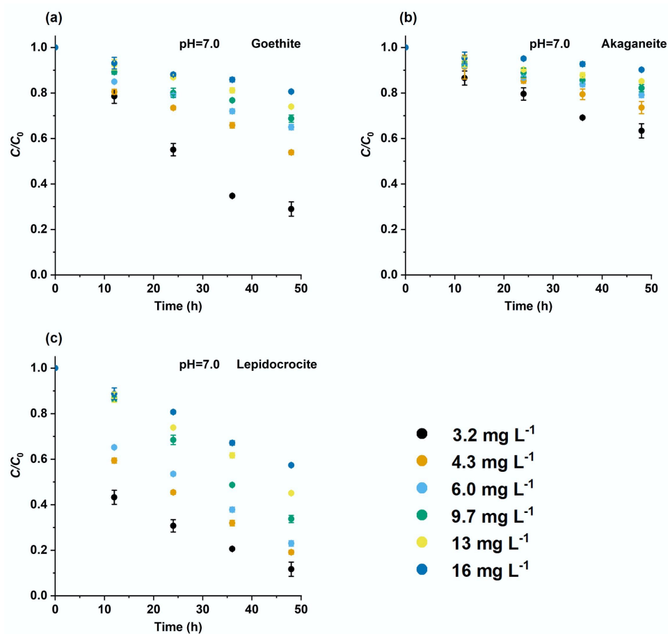
Supplementary Fig. S8 Catalytic hydrolysis kinetics of pNPP with different initial concentrations by different nanomaterials: (a) goethite, (b) akaganeite, and (c) lepidocrocite at pH 7.0.
