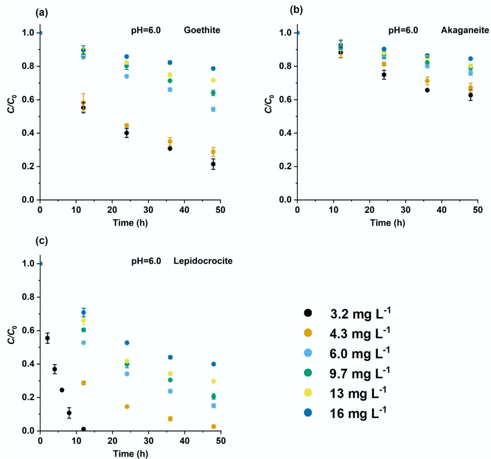
Supplementary Fig. S7 Catalytic hydrolysis kinetics of pNPP with different initial concentrations by different nanomaterials: (a) goethite, (b) akaganeite, and (c) lepidocrocite at pH 6.0.
