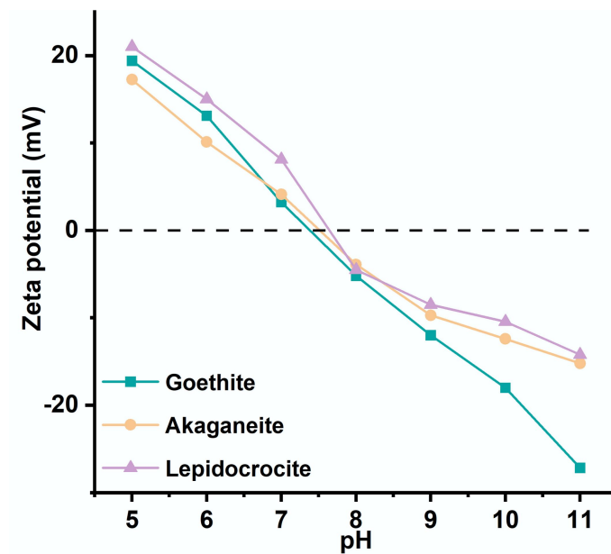
Supplementary Fig. S5 Zeta potential of goethite, akaganeite, and lepidocrocite at different pH values.
