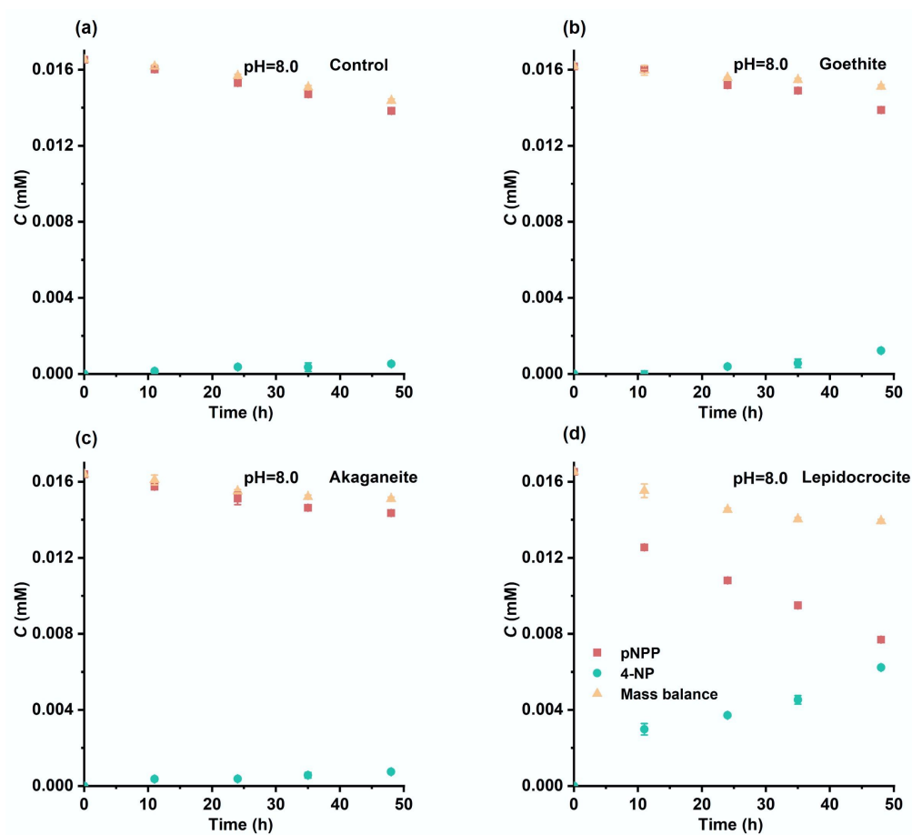
Supplementary Fig. S4 Changes of pNPP and 4-NP concentrations during pNPP hydrolysis experiments at pH 8.0 in (a) control, (b) goethite, (c) akaganeite, and (d) lepidocrocite. Error bars indicate standard deviations of triplicates.
