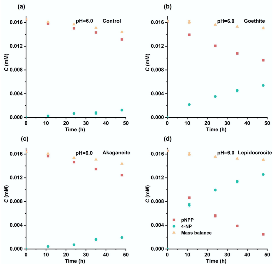
Supplementary Fig. S2 Changes of pNPP and 4-NP concentrations during pNPP hydrolysis experiments at pH 6.0 in (a) control, (b) goethite, (c) akaganeite, and (d) lepidocrocite. Error bars indicate standard deviations of triplicates.
