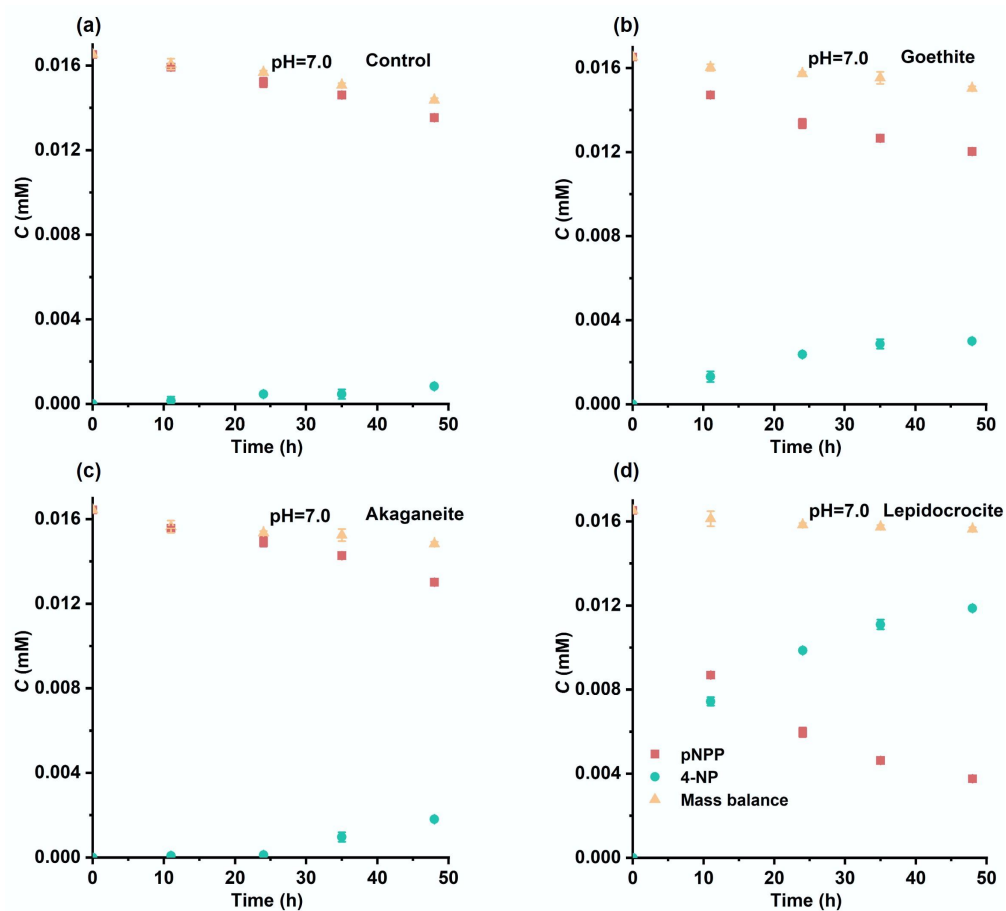
Supplementary Fig. S3 Changes of pNPP and 4-NP concentrations during pNPP hydrolysis experiments at pH 7.0 in (a) control, (b) goethite, (c) akaganeite, and (d) lepidocrocite. Error bars indicate standard deviations of triplicates.
