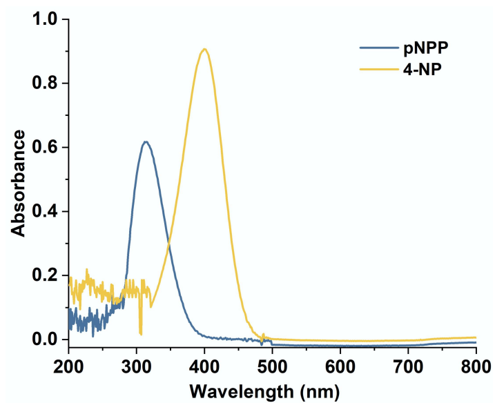
Supplementary Fig. S1 The UV-vis spectra of pNPP and 4-NP under alkaline conditions
