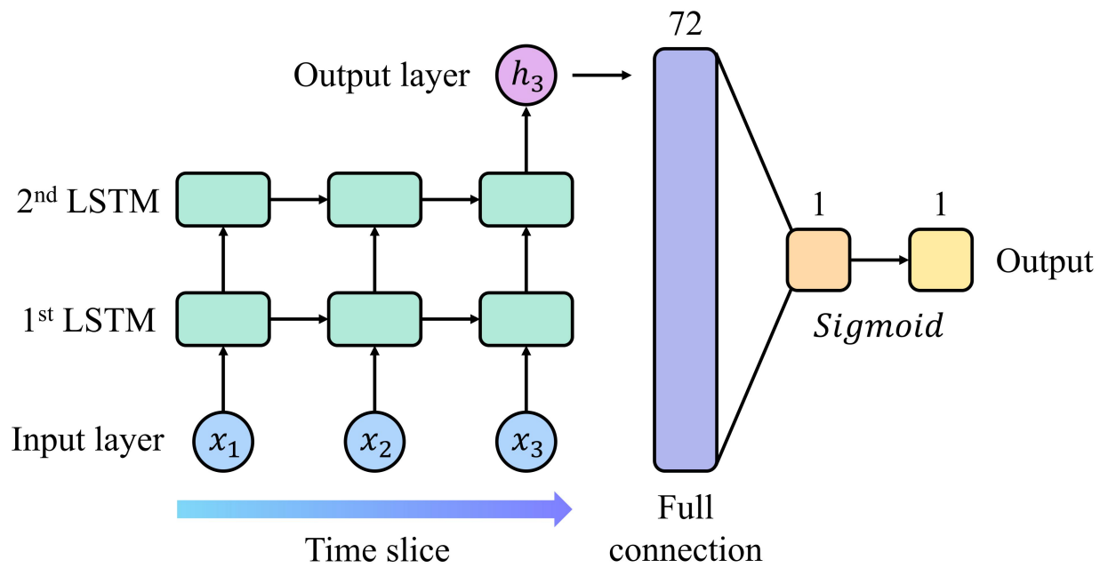
Fig. 3 Structure of LSTM.
