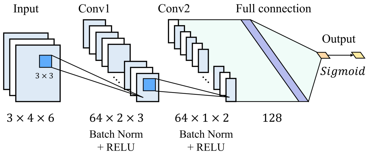
Fig. 2 Structure of CNN.
