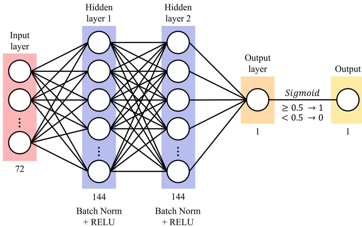
Fig. 1 Structure of MLP.
