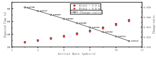
(e) width of target corridor is 3.9m, width of prior corridor is 4.0m
