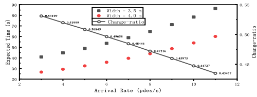
(a) width of target corridor is 3.5m, width of prior corridor is 4.0m
