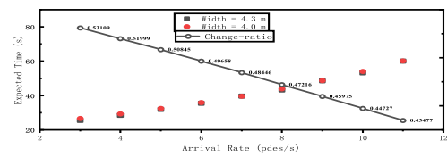
(h) width of target corridor is 4.3m, width of prior corridor is 4.0m
