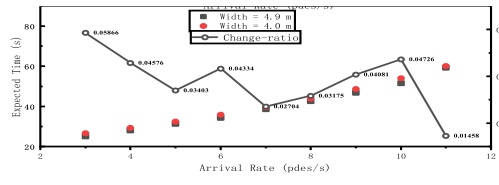
(n) width of target corridor is 4.9m, width of prior corridor is 4.0m
