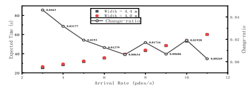
(i) width of target corridor is 4.4m, width of prior corridor is 4.0m
