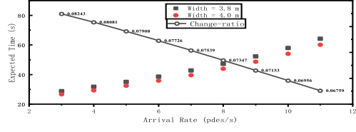
(d) width of target corridor is 3.8m, width of prior corridor is 4.0m
