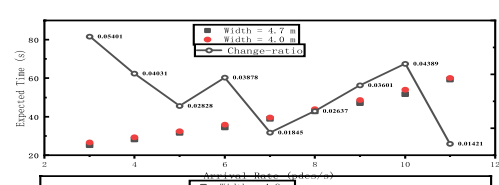
(l) width of target corridor is 4.7m, width of prior corridor is 4.0m
