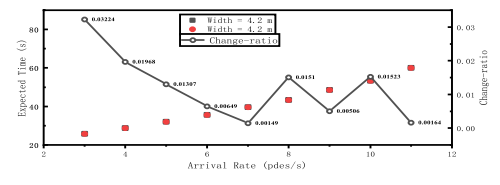
(g) width of target corridor is 4.2m, width of prior corridor is 4.2m
