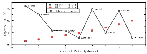
(f) width of target corridor is 4.1m, width of prior corridor is 4.0m
