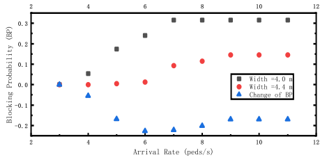
(j) width of target corridor is 4.0m, width of prior corridor is 4.4m
