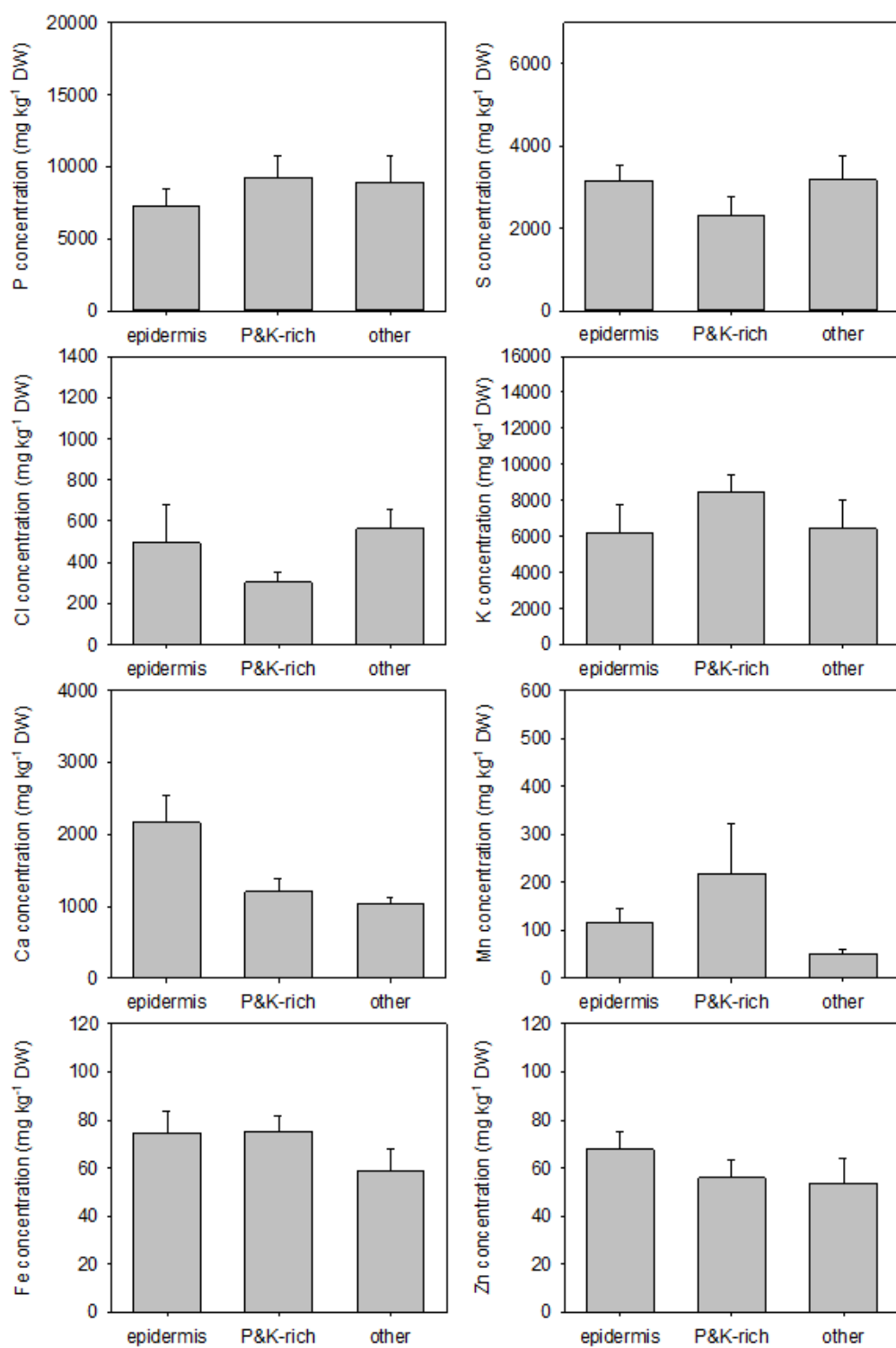
Supplementary Figure S1. Cell-type specific concentrations of phosphorus (P), sulphur (S), chlorine (Cl), potassium (K), calcium (Ca), manganese (Mn), iron (Fe) and zinc (Zn) in longitudinal sections of Lupinus pilosus seed. Shown are means + standard errors ( n_{\text{epidermis}} = 2 , n_{\text{P\&K-rich}} = 6 , n_{\text{other}} = 6 ).
