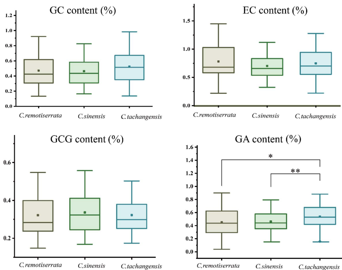
Figure S2 Box plot comparison of catechin components among the three tea groups
