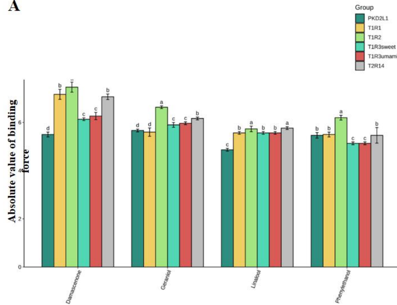
Fig. S1 (A) Histogram of binding force between volatiles and taste receptors contributing to honey aroma (B) Electronic tongue validation chart with missing experimental review results
