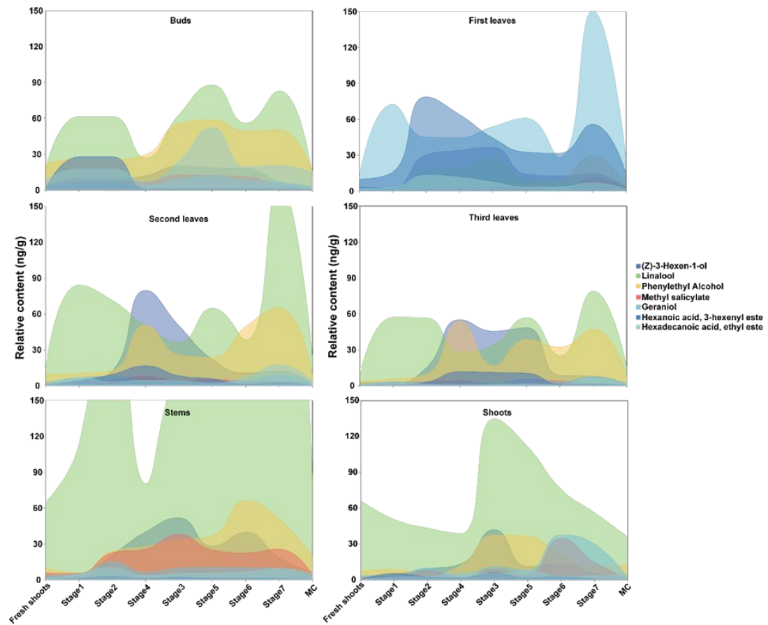
Supplementary Fig. 9. The changes in the content of the five continuously emission compounds of 'ZL22' different tissues during the withering periods. MC, the tea products.
