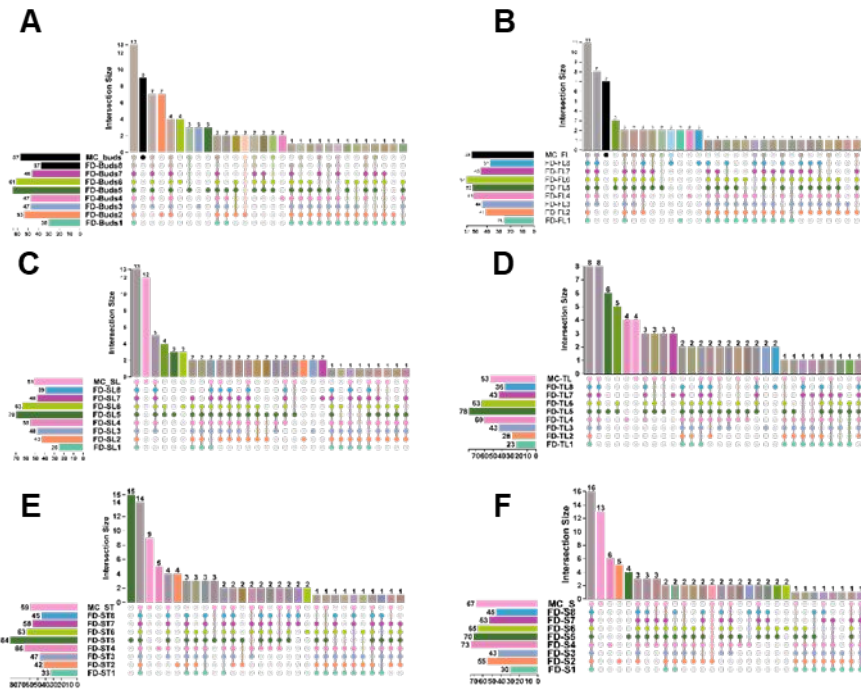
Supplementary Fig. 3. The upset plot of ‘FD’ buds (A), first leaves (B), second leaves (C), third leaves (D), the stems (E), and tea shoots (F) during the withering period, respectively.
