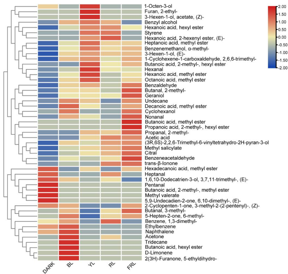
Fig. S2. Cluster analysis of key aromatic components in Sangzhi White Tea under different light quality withering.
