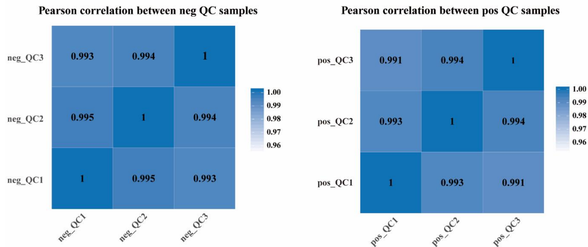
Fig.S2. Pearson correlation heatmap of metabolite relative quantification values in quality control (QC) samples under positive and negative ionization modes
