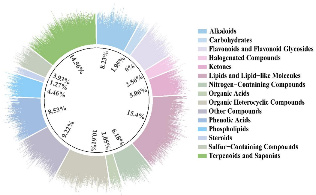
Fig.S1. Donut chart of non-volatile metabolite class proportions across five Minnan oolong tea cultivars
