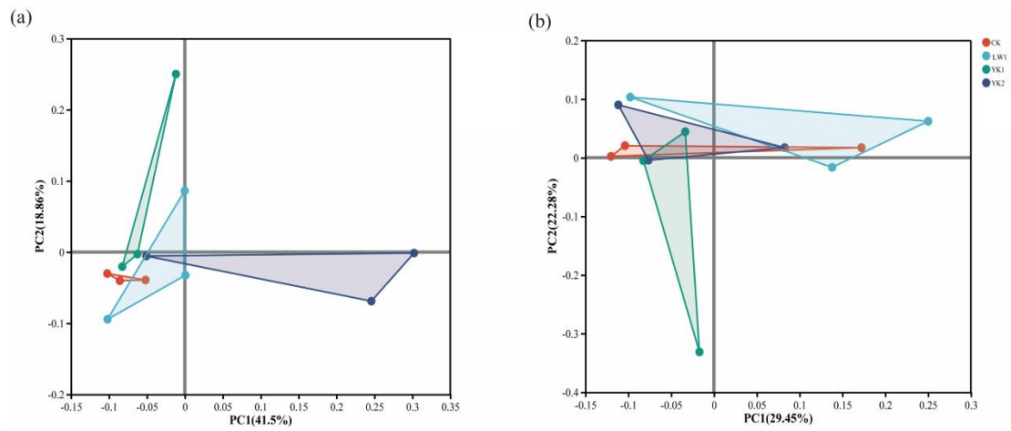
Figure S1. Multivariate Ordination Analysis of Bacterial and Fungal Community Structures in Tea Plantation Soils. PCoA of Bacterial Communities(a); PCoA of Fungal Communities(b). CK (no biochar), LW1(0.5% reed biochar), YK1(0.5% coconut shell biochar), YK2(1.0% coconut shell biochar).
