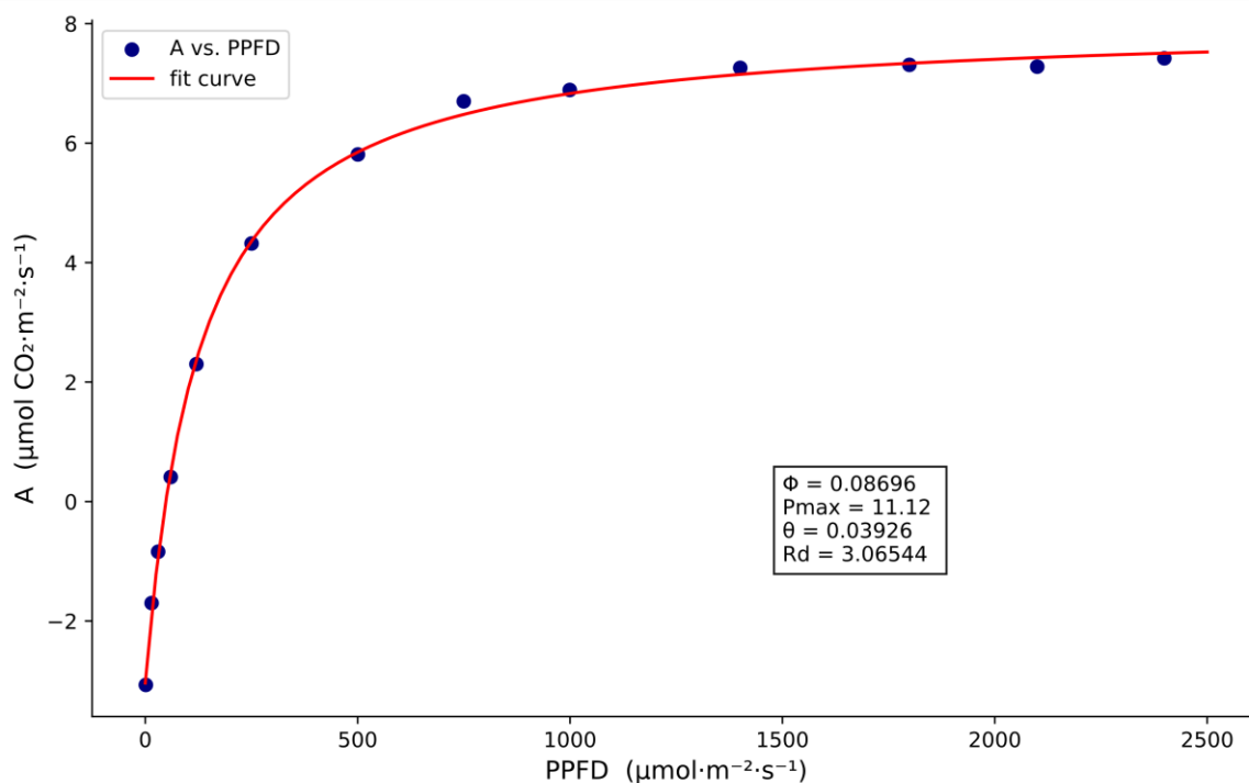
Figure S3. Photosynthetic light-response curve showing the relationship between leaf photosynthetic rate and PPFD, with model fit (red curve) and measured data (blue dots), demonstrating light saturation characteristics. The curve demonstrates the progressive increase in photosynthetic rate with rising PPFD, asymptotically approaching a plateau, which reflects the light saturation phenomenon in plant photosynthesis.
