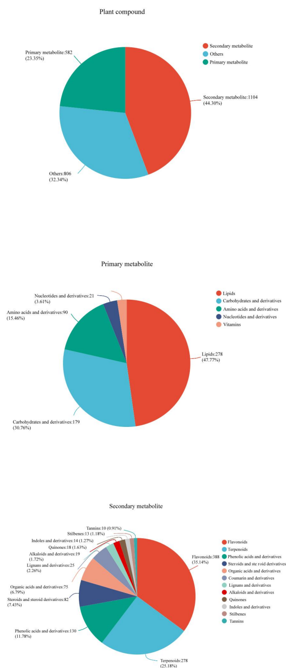
Fig S1. Classification of the whole metabolites, classification of primary metabolites, and classification of secondary metabolites in both EST and ESO. EST and ESO represent the tender leaf or older leaf of E Se tea, respectively.
