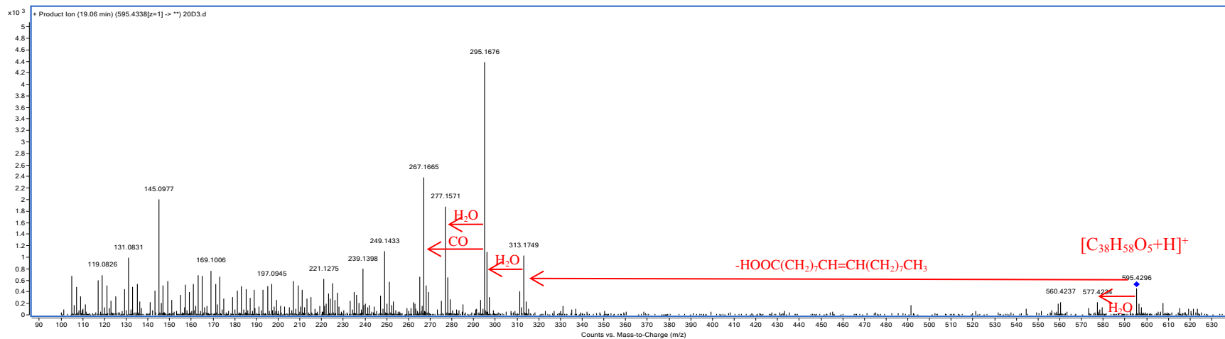
Figure S18 The MS spectra for 5.
