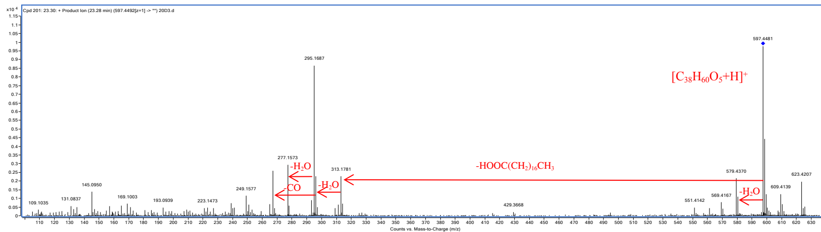
Figure S14 The MS spectra for 1 .
