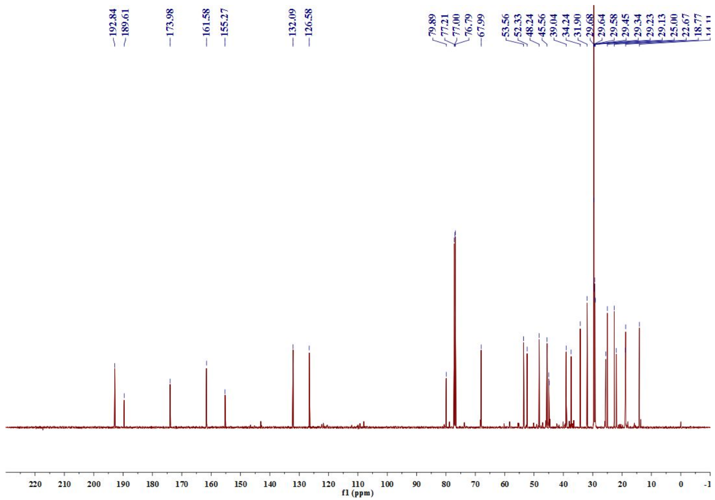
Figure S12 13 C NMR spectra of 3
