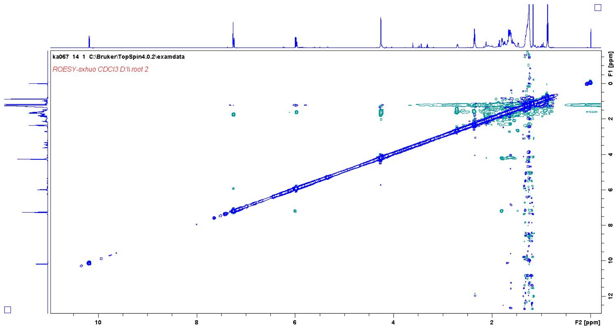
Figure S10 ROESY spectra of 2 .
