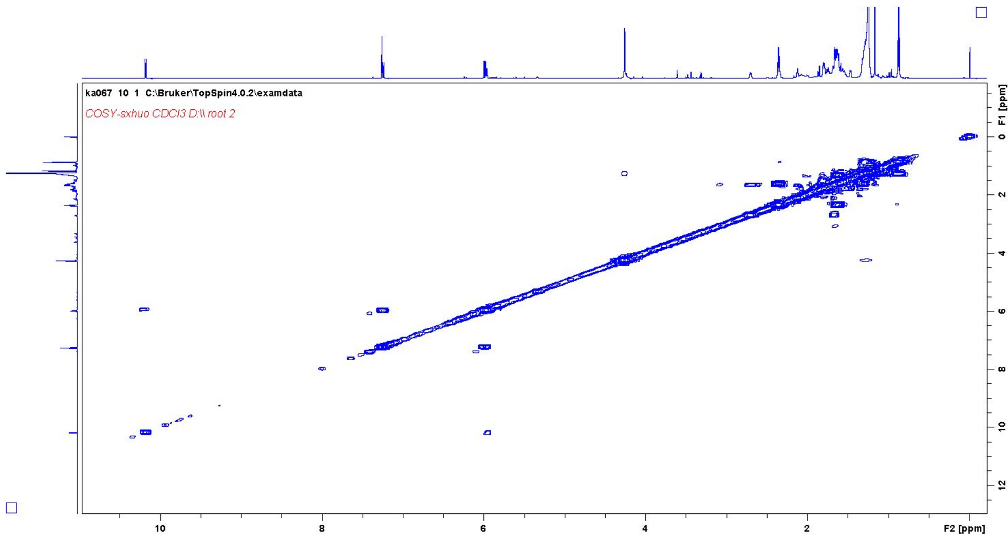
Figure S8 ^1\text{H} ^1\text{H} COSY spectra of 2 .
