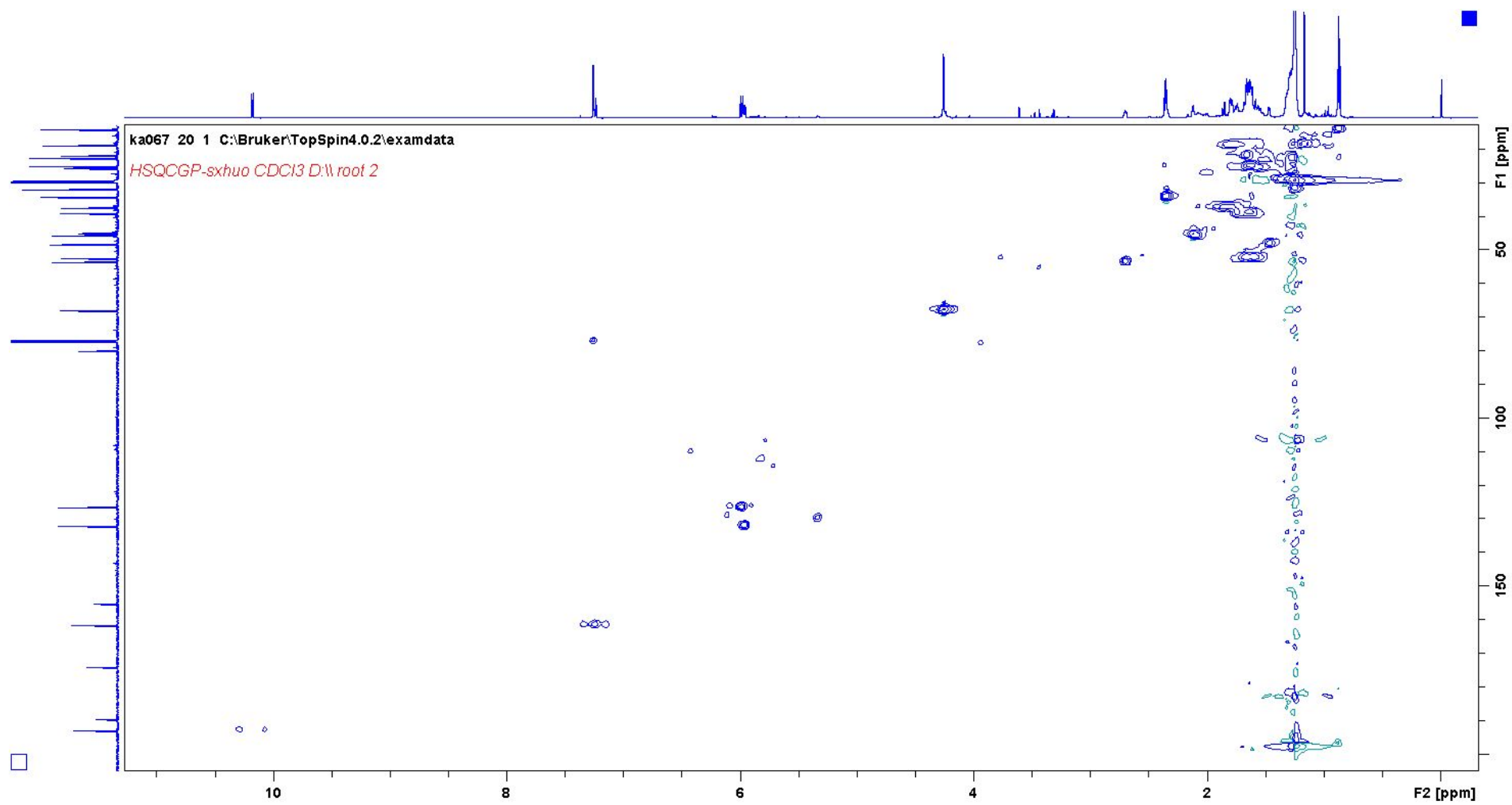
Figure S7 HSQC spectra of 2 .
