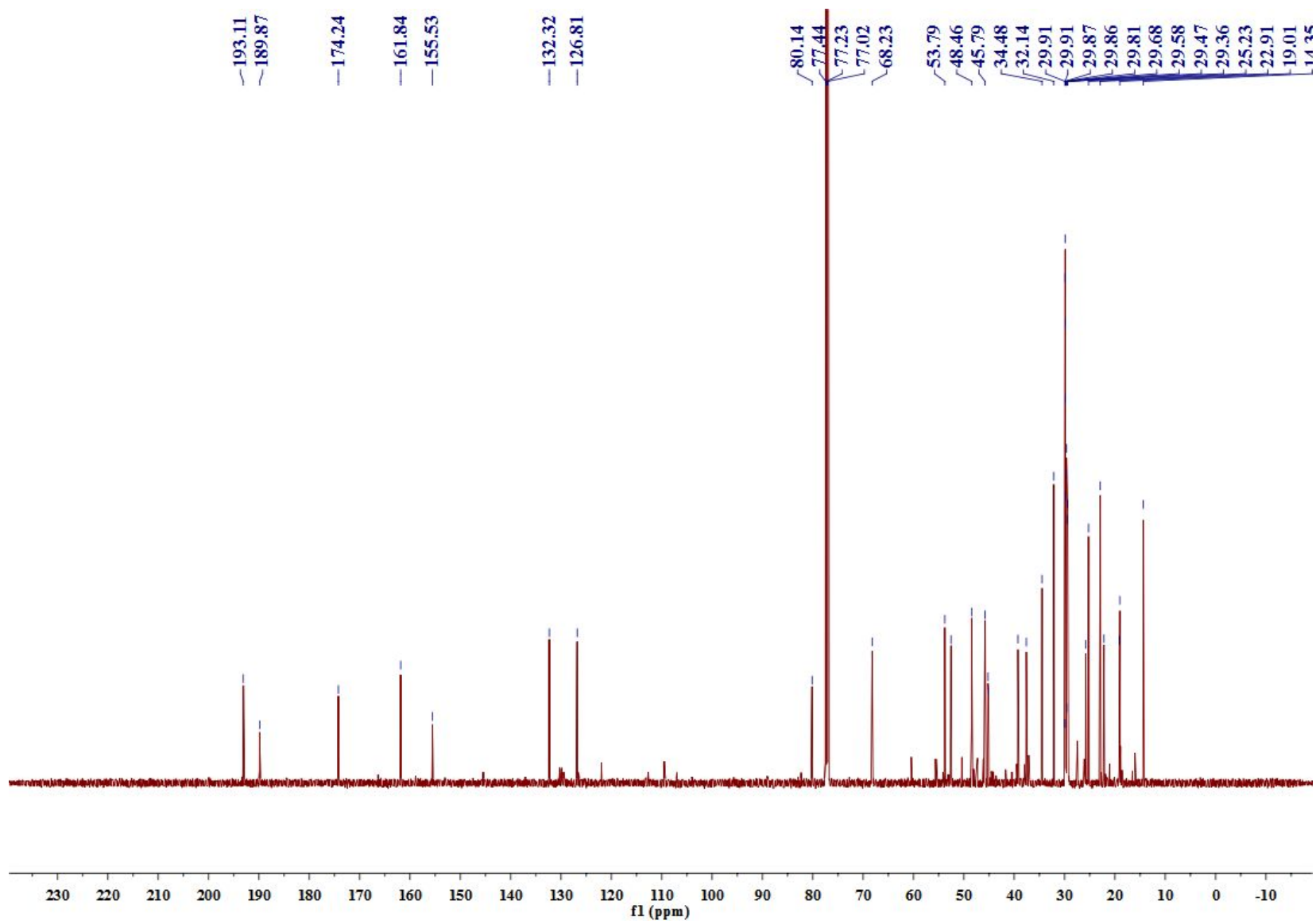
Figure S6 13 C NMR spectra of 2
