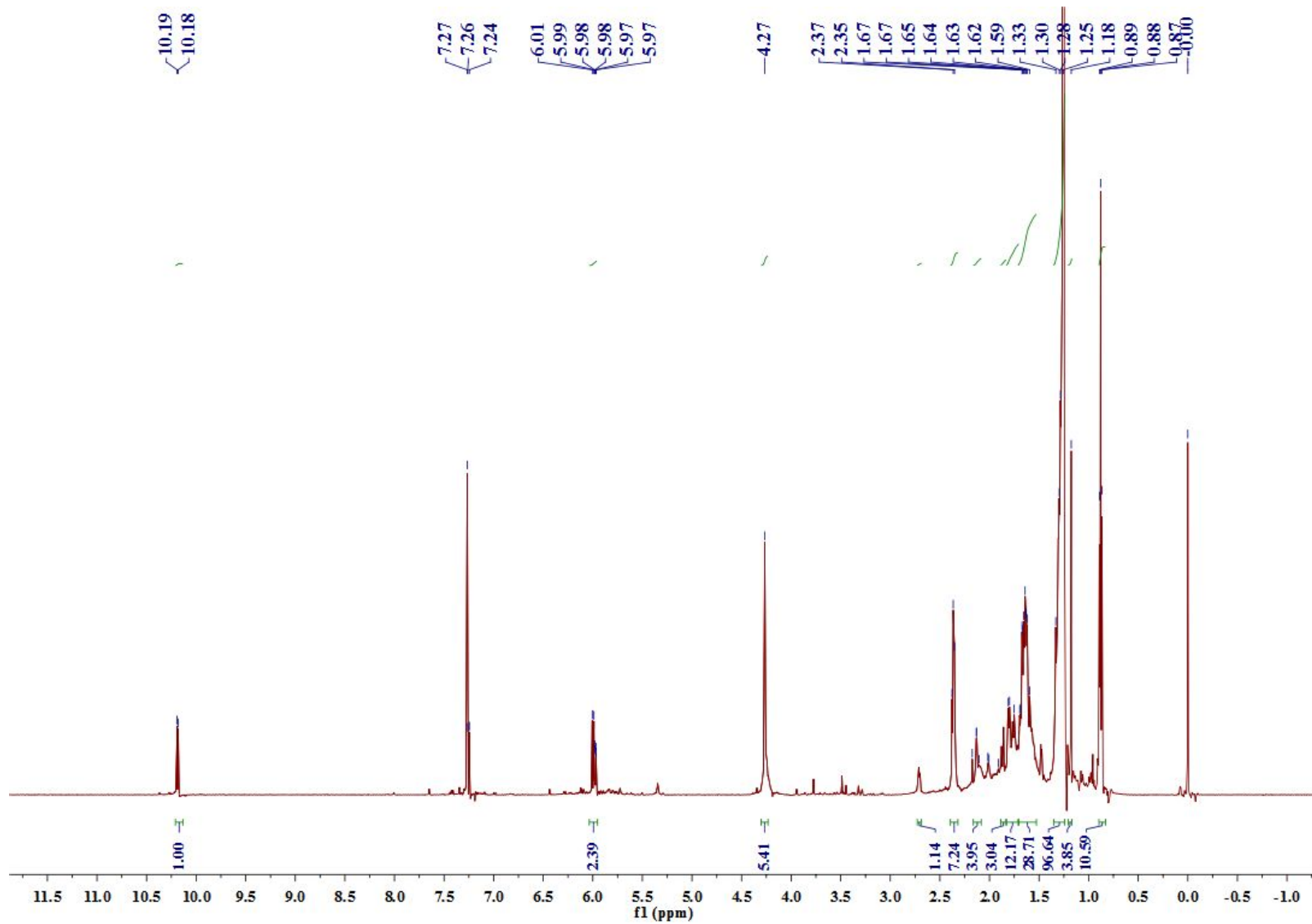
Figure S5 1 H NMR spectra of 2
