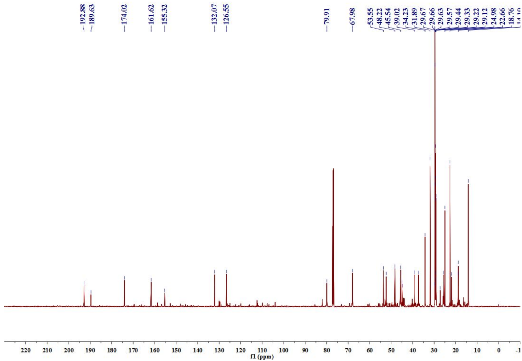
Figure S4 13 C NMR spectra of 1
