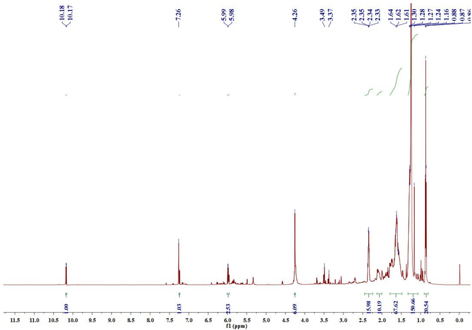
Figure S3 ^1\text{H} NMR spectra of 1
