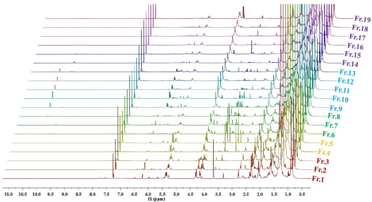
Figure S1 1 H NMR spectra of Fr.1-19.
