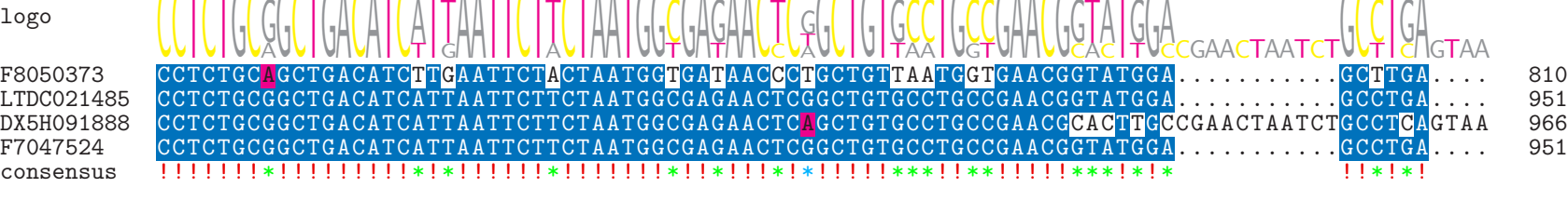
Supplementary Fig. S3 CDS sequence comparison of CsJAZ12 .
