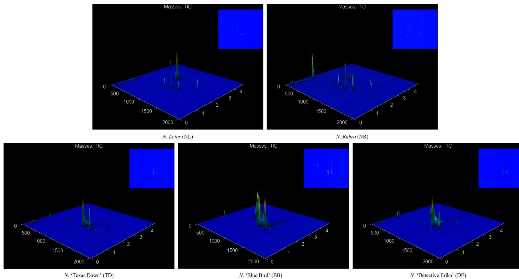
Figure S4. The spectrogram of volatile components in five water lily samples obtained from GC×GC-TOFMS.
