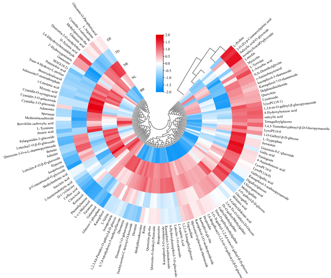
Figure S2. Heatmap of crucially changed differential non-volatile metabolites in five water lily samples.
