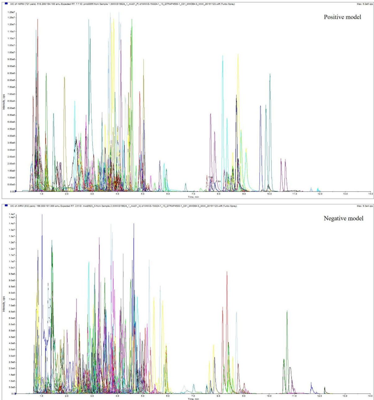
Figure S1. The spectrogram of non-volatile components in five water lily samples obtained from UPLC-MS/MS.
