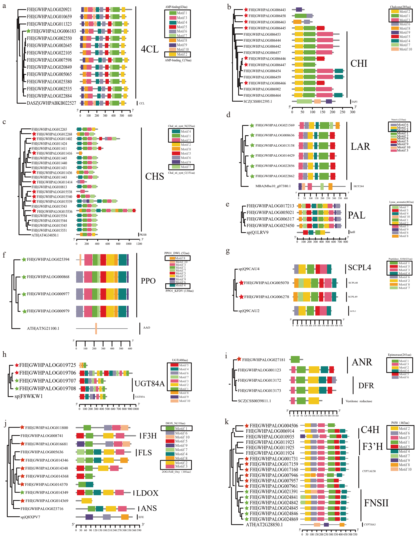
Supplemental Fig S22. Comparison of results from Gfanno and KAAS annotation methods using F. hispida genome. Green stars indicate more correctly annotated genes by Gfanno than by KAAS, and red stars indicate incorrectly annotated genes by KAAS.
