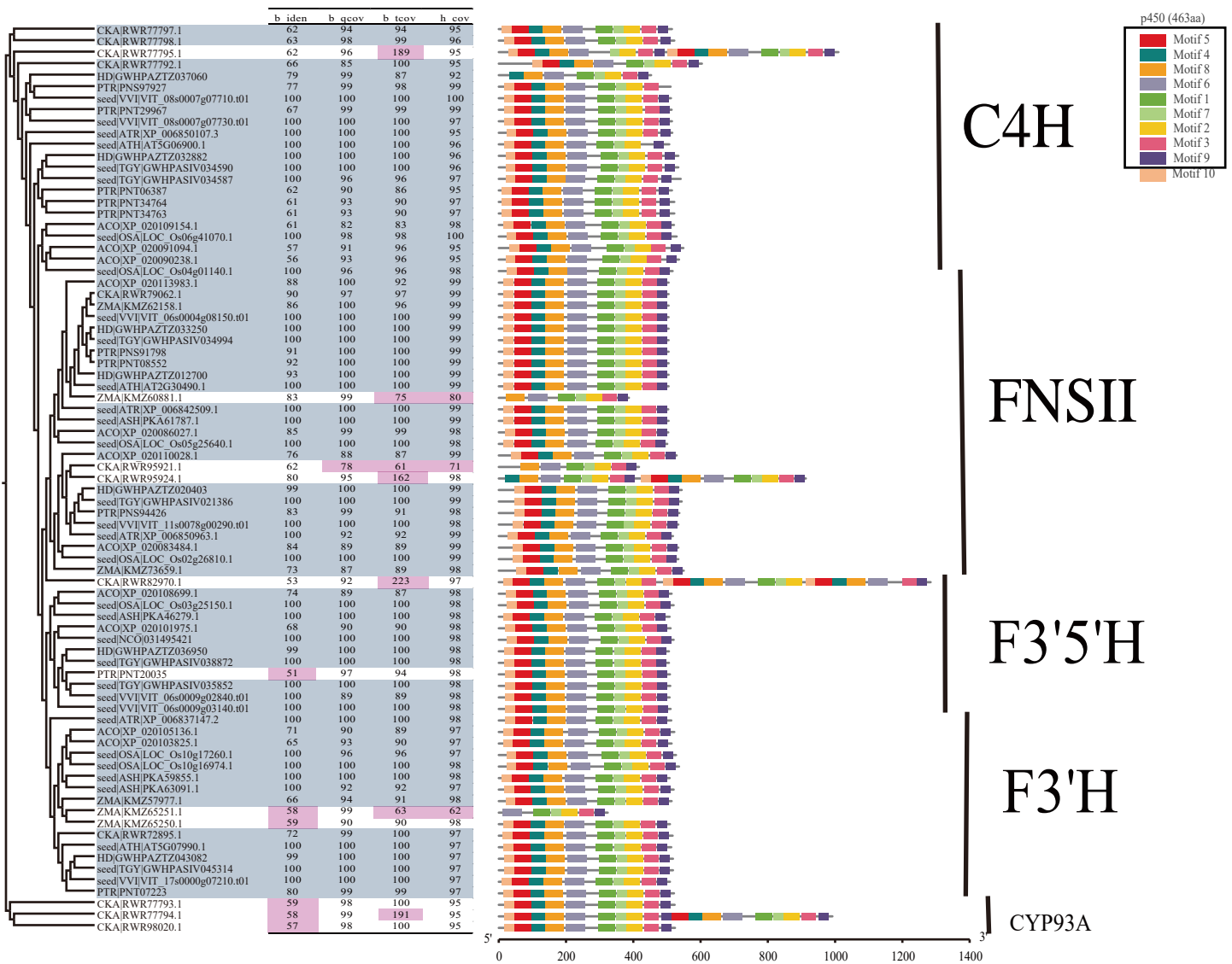
Fig S11. The parameter validation for C4H, FNS II, F3'H, and F3'5'H in CYP450 superfamily.
