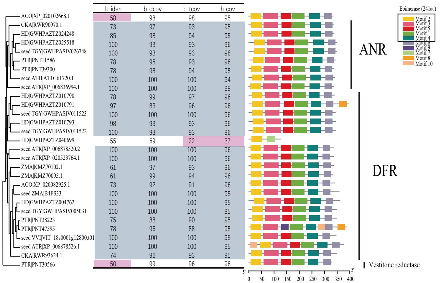
Fig S10. The parameter selection for ANR and DFR in SDR superfamily of the test species.
